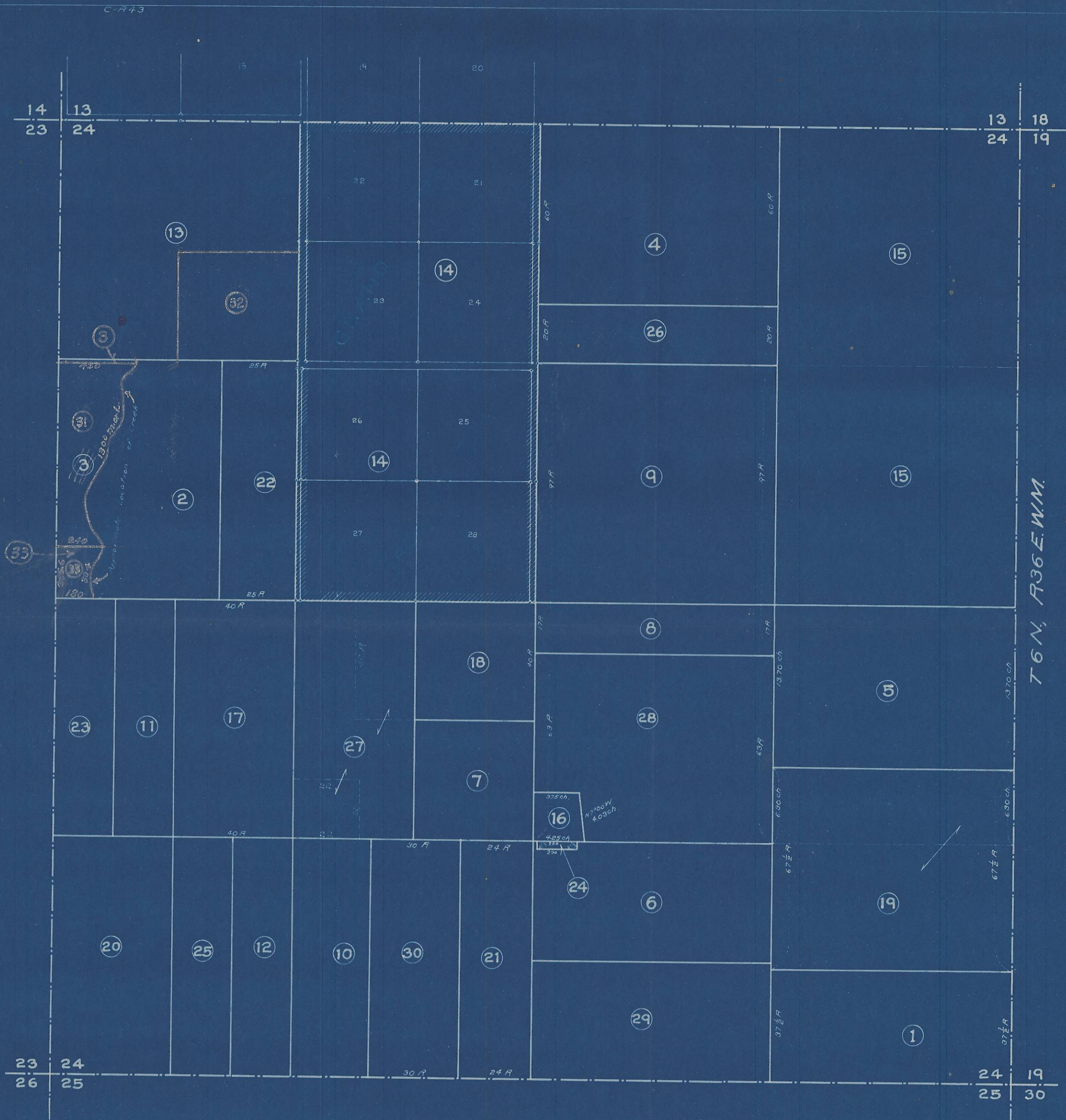
Section 24 Tp 6 N, R 35 E. W.M. Scale 1 inch = 500 feet.
