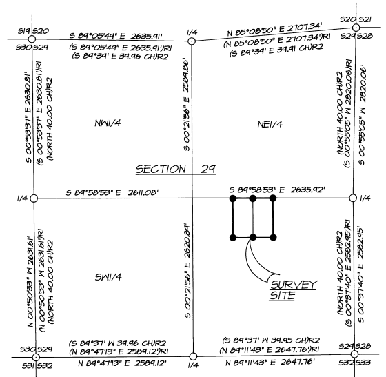
SECTION CONTROL DIAGRAM
