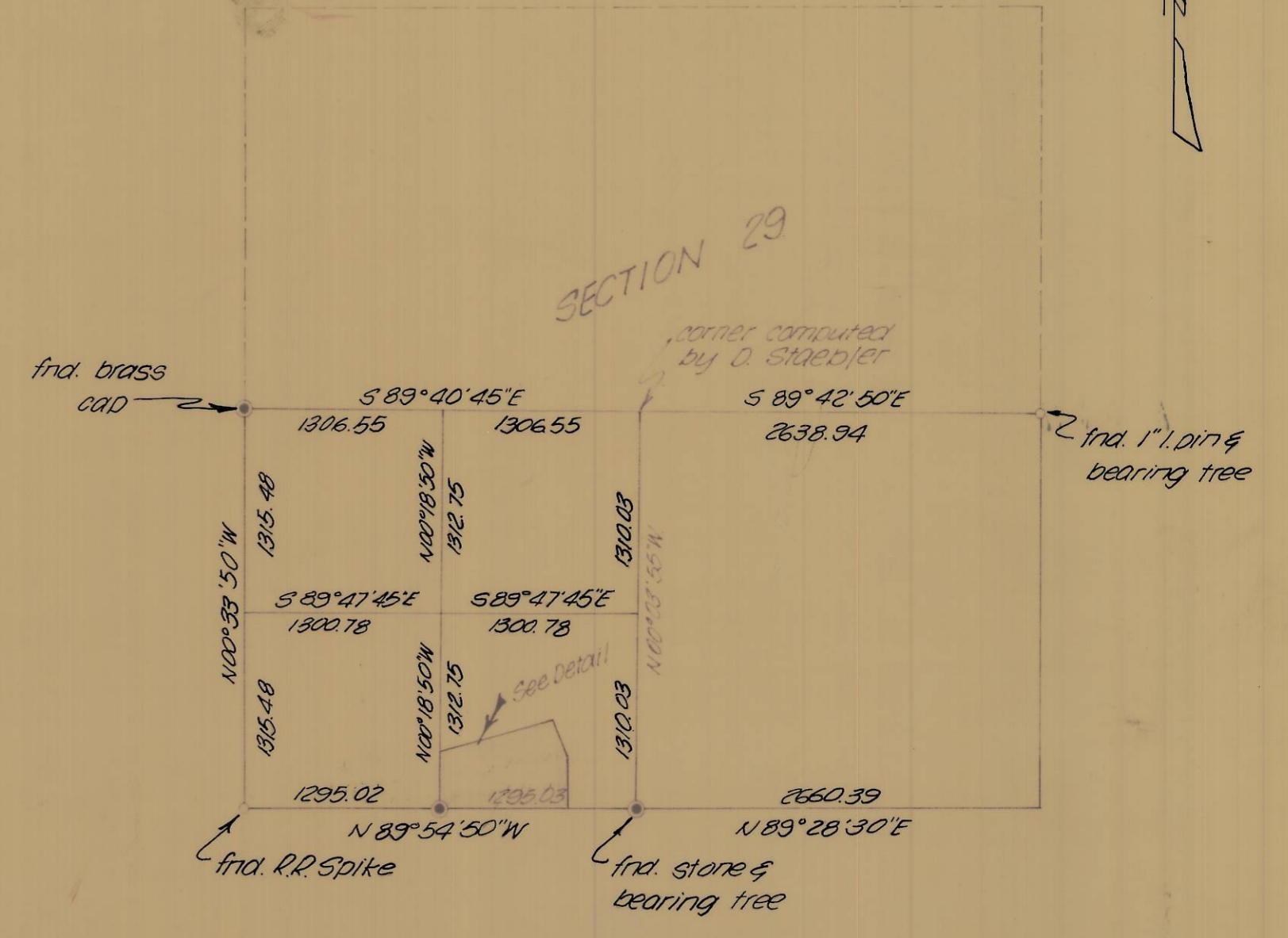
SECTION BREAKDOWN 1" = 100'
